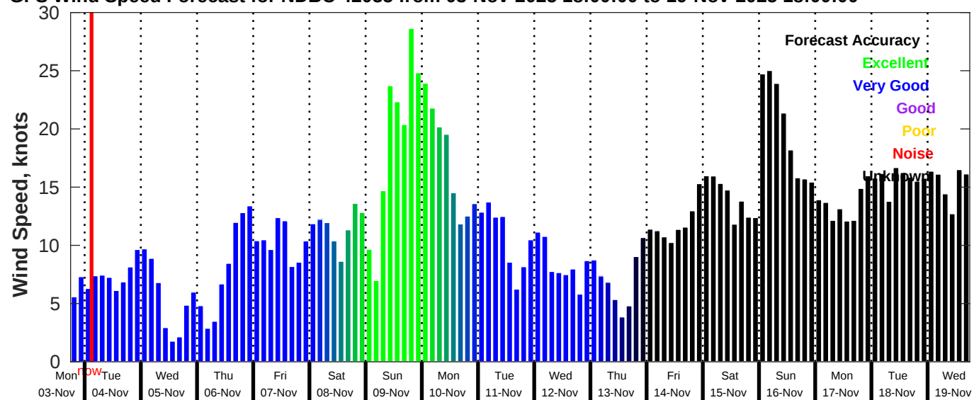
GFS Wind Speed Forecast for NDBC 42035 from 03-Nov-2025 18:00:00 to 19-Nov-2025 18:00:00
