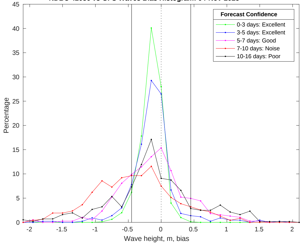
NDBC 42036 vs GFS Waves Bias Histogram: 04-Nov-2025
