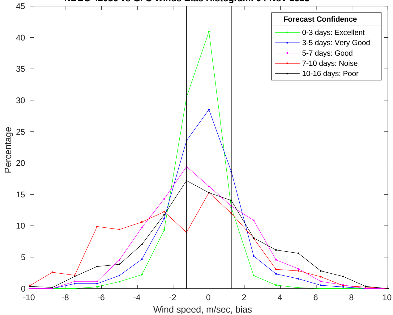
NDBC 42036 vs GFS Winds Bias Histogram: 04-Nov-2025
