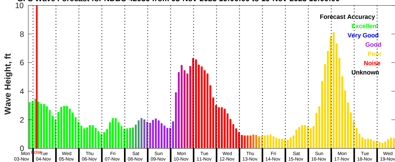
GFS Wave Forecast for NDBC 42036 from 03-Nov-2025 19:00:00 to 19-Nov-2025 19:00:00
