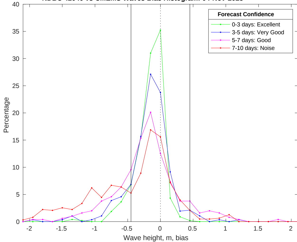
NDBC 42040 vs CMEMS Waves Bias Histogram: 04-Nov-2025
