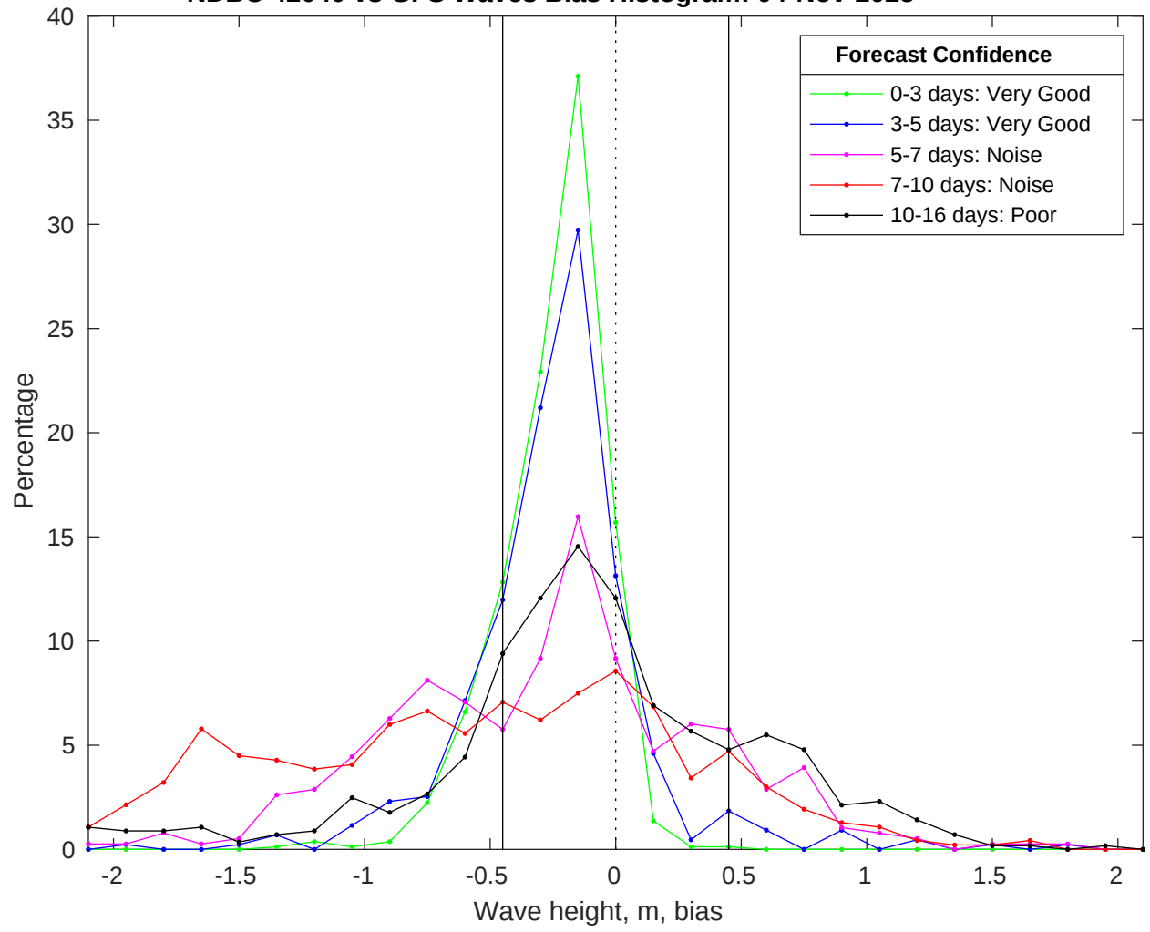
NDBC 42040 vs GFS Waves Bias Histogram: 04-Nov-2025
