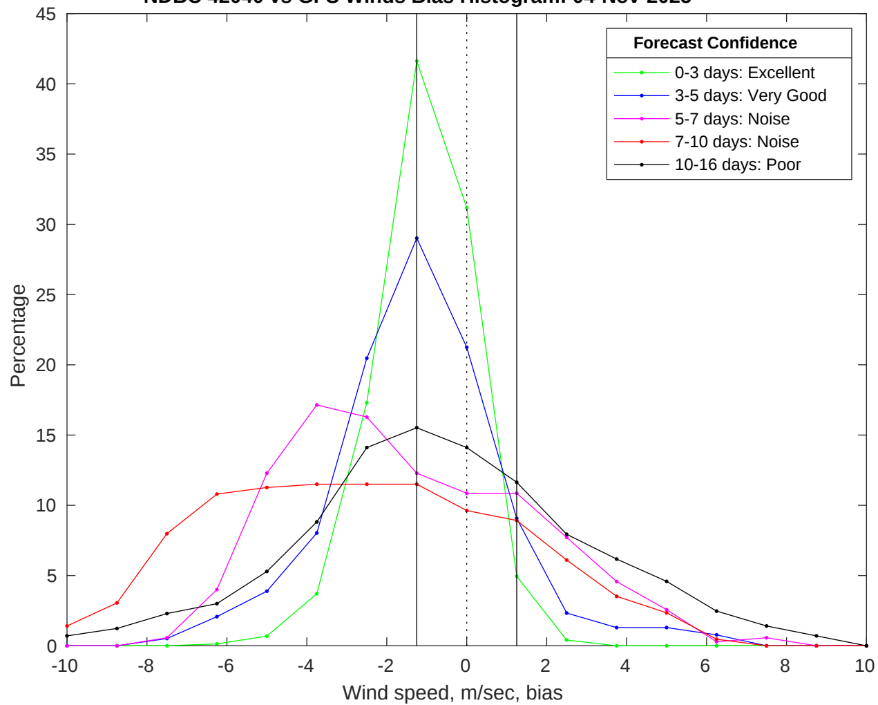
NDBC 42040 vs GFS Winds Bias Histogram: 04-Nov-2025
