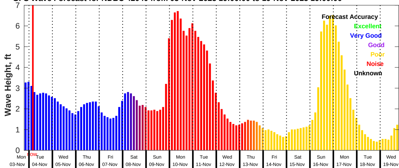
GFS Wave Forecast for NDBC 42040 from 03-Nov-2025 19:00:00 to 19-Nov-2025 19:00:00
