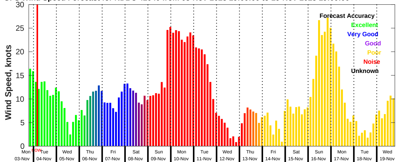
GFS Wind Speed Forecast for NDBC 42040 from 03-Nov-2025 19:00:00 to 19-Nov-2025 19:00:00
