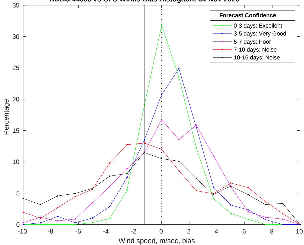
NDBC 44008 vs GFS Winds Bias Histogram: 04-Nov-2025
