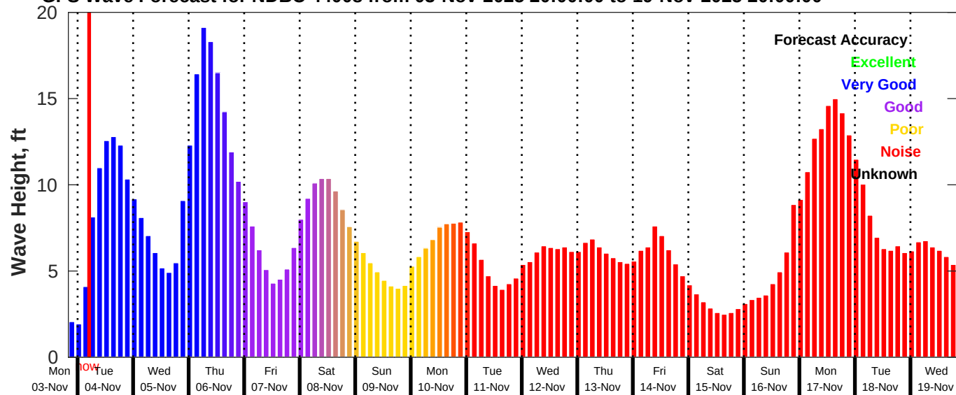
GFS Wave Forecast for NDBC 44008 from 03-Nov-2025 20:00:00 to 19-Nov-2025 20:00:00
