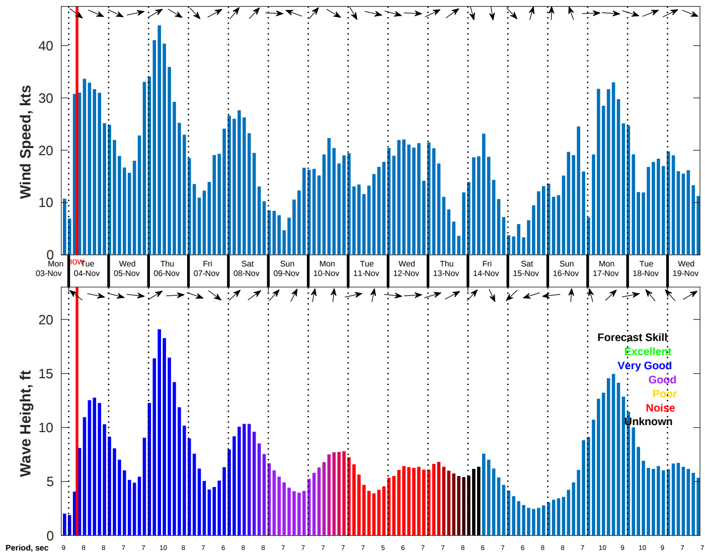
Wind & Wave Forecast for NDBC 44008 from 03-Nov-2025 20:00:00 to 19-Nov-2025 20:00:00
