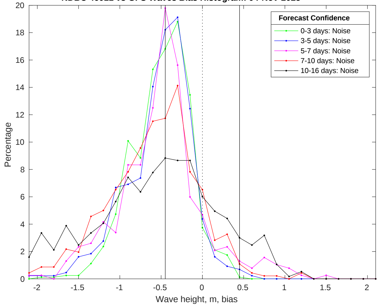
NDBC 46011 vs GFS Waves Bias Histogram: 04-Nov-2025
