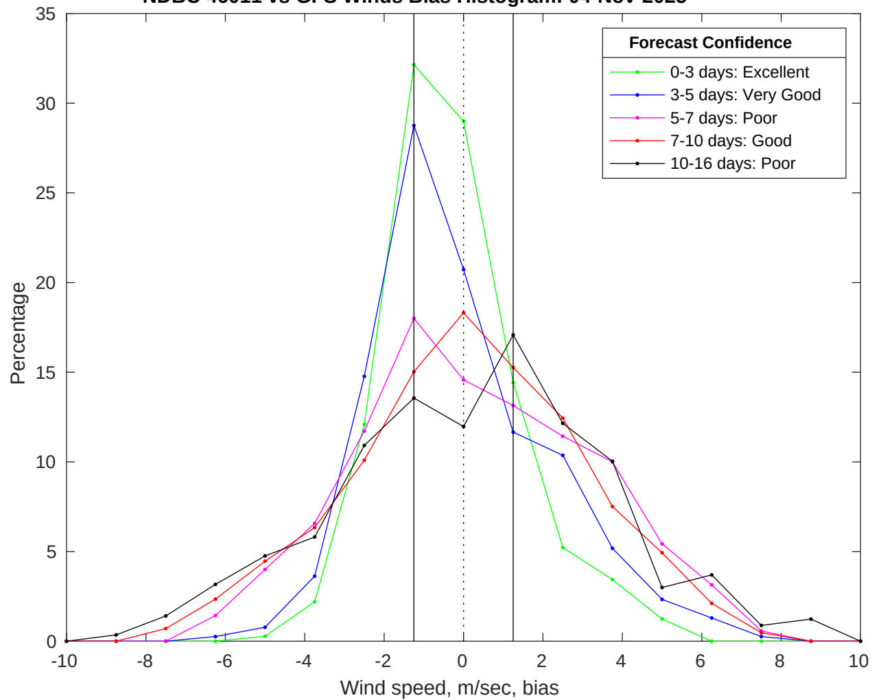
NDBC 46011 vs GFS Winds Bias Histogram: 04-Nov-2025
