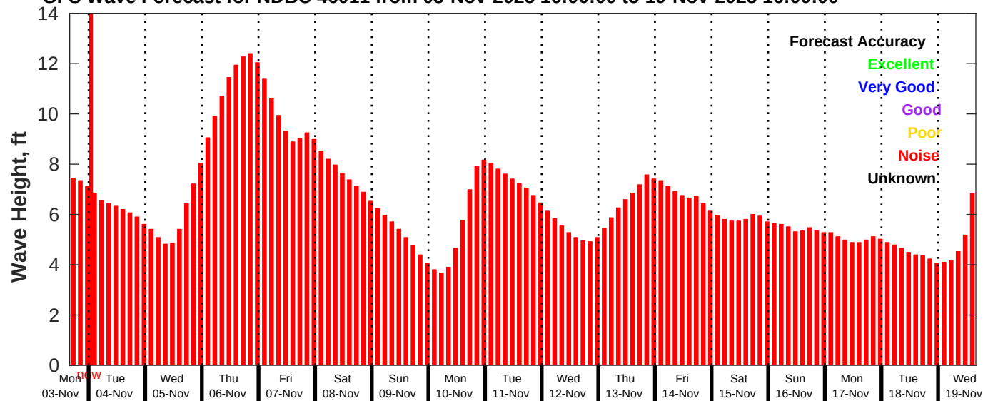
GFS Wave Forecast for NDBC 46011 from 03-Nov-2025 16:00:00 to 19-Nov-2025 16:00:00
