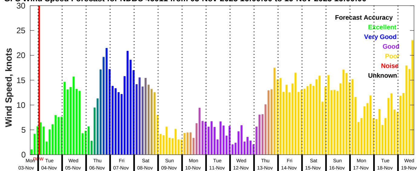
GFS Wind Speed Forecast for NDBC 46011 from 03-Nov-2025 16:00:00 to 19-Nov-2025 16:00:00
