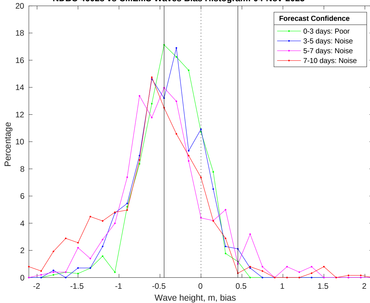
NDBC 46028 vs CMEMS Waves Bias Histogram: 04-Nov-2025
