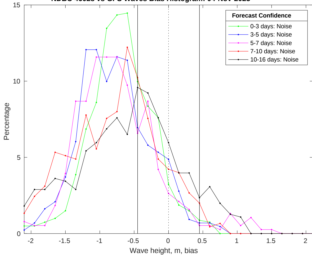
NDBC 46028 vs GFS Waves Bias Histogram: 04-Nov-2025
