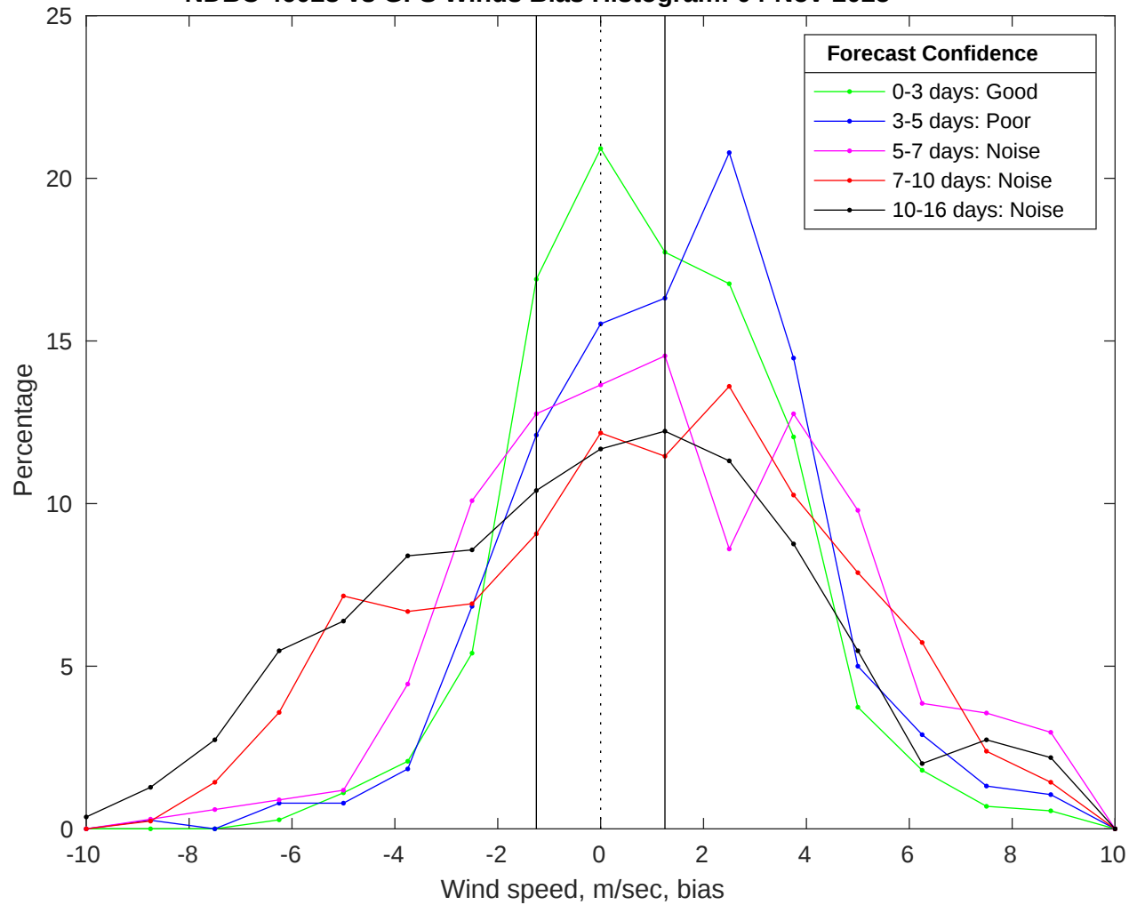
NDBC 46028 vs GFS Winds Bias Histogram: 04-Nov-2025
