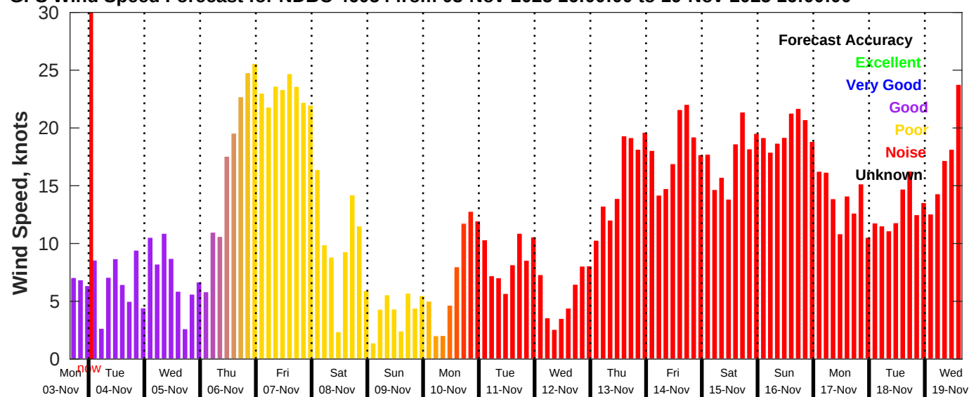
GFS Wind Speed Forecast for NDBC 46054 from 03-Nov-2025 16:00:00 to 19-Nov-2025 16:00:00
