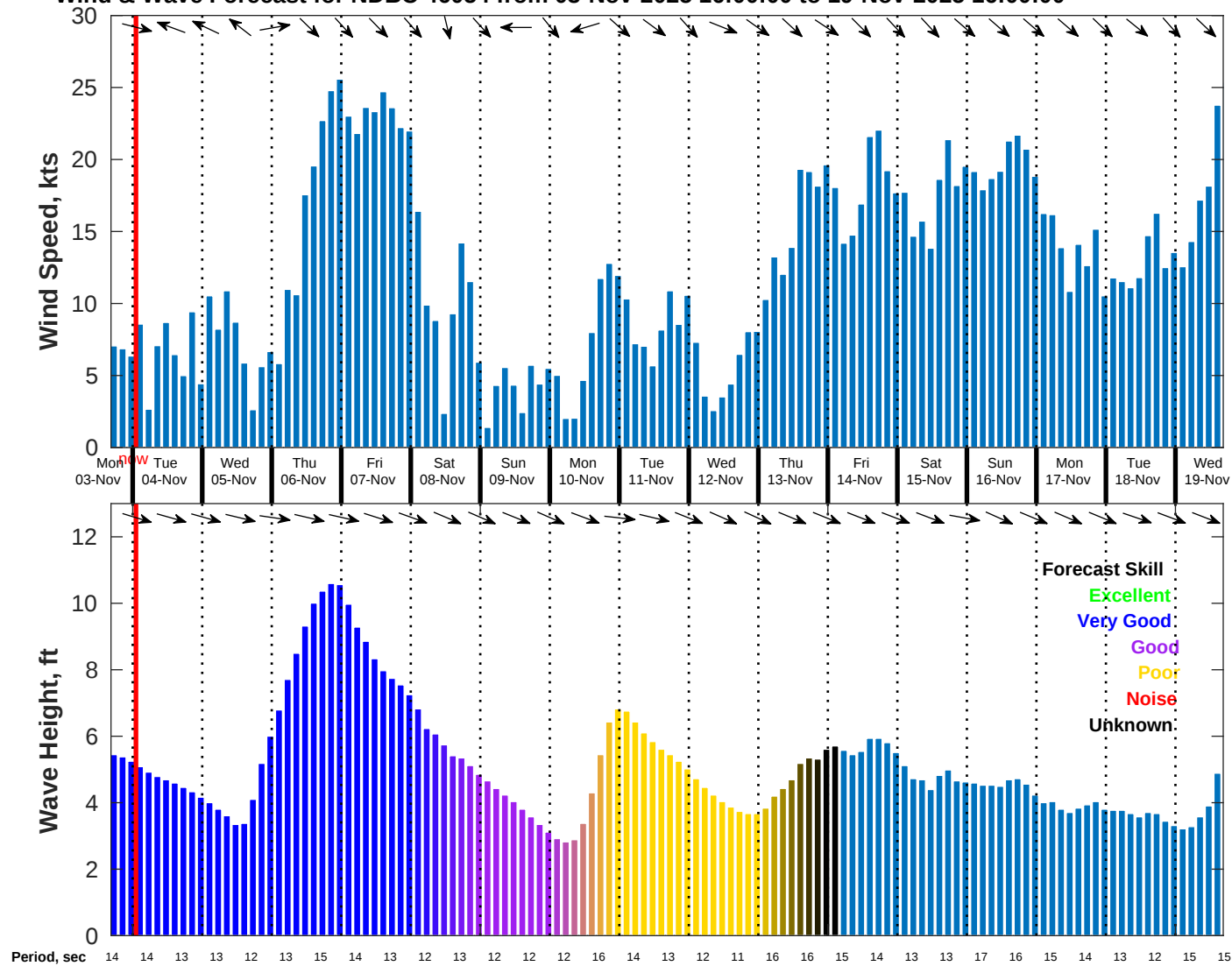
Wind & Wave Forecast for NDBC 46054 from 03-Nov-2025 16:00:00 to 19-Nov-2025 16:00:00
