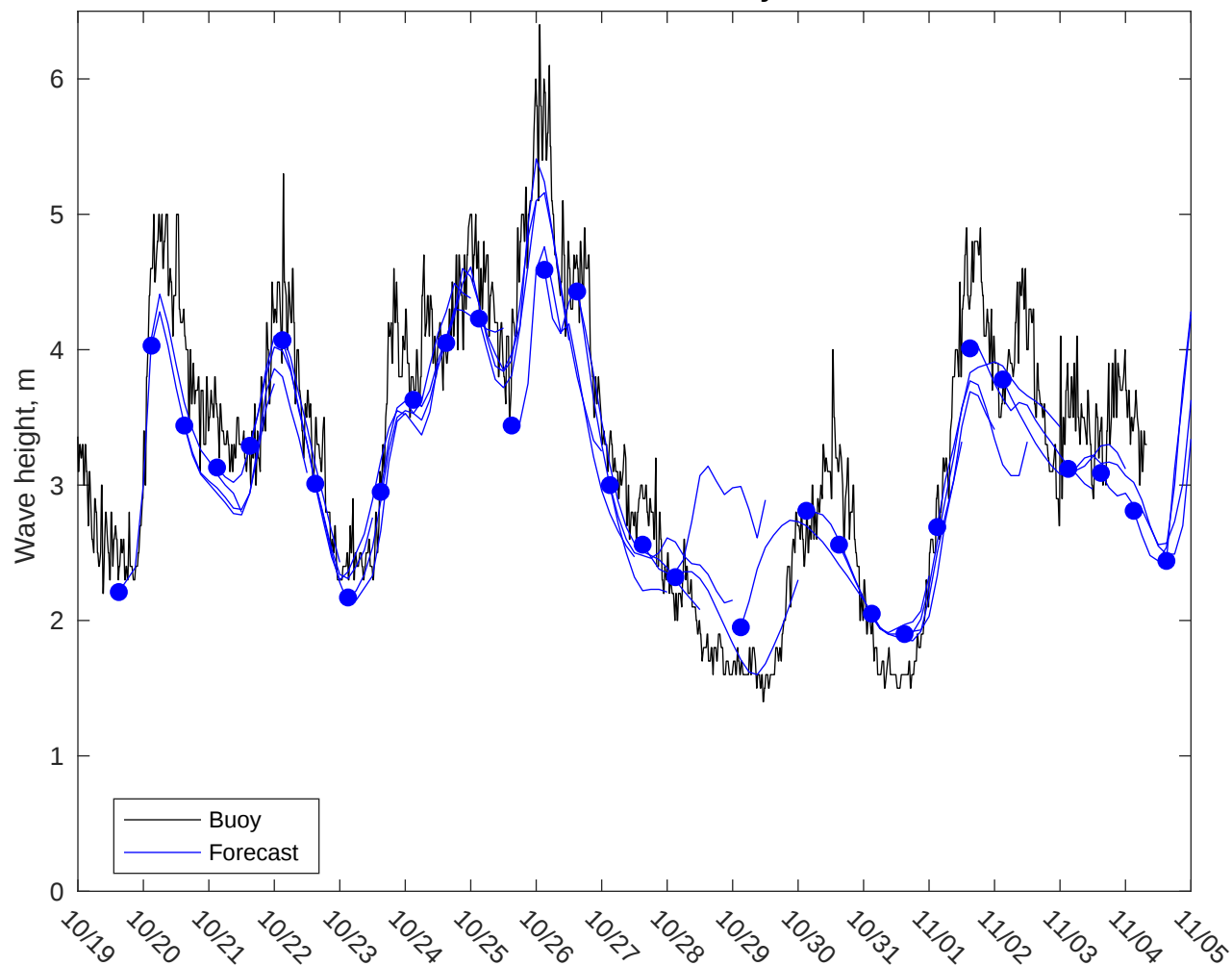
NDBC 46059 vs GFS Waves: 3 to 5 day forecast
