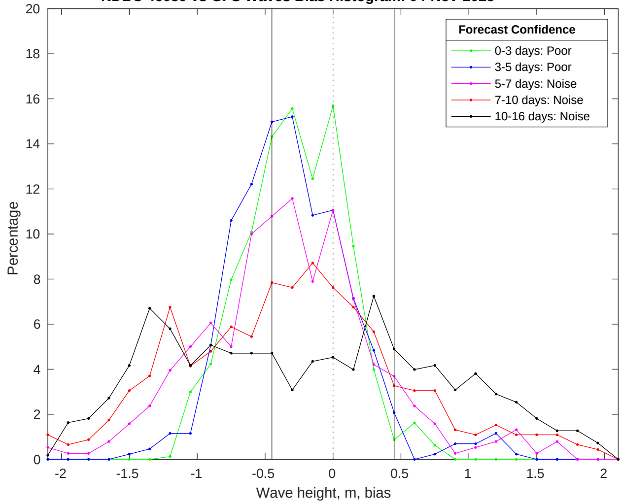
NDBC 46059 vs GFS Waves Bias Histogram: 04-Nov-2025
