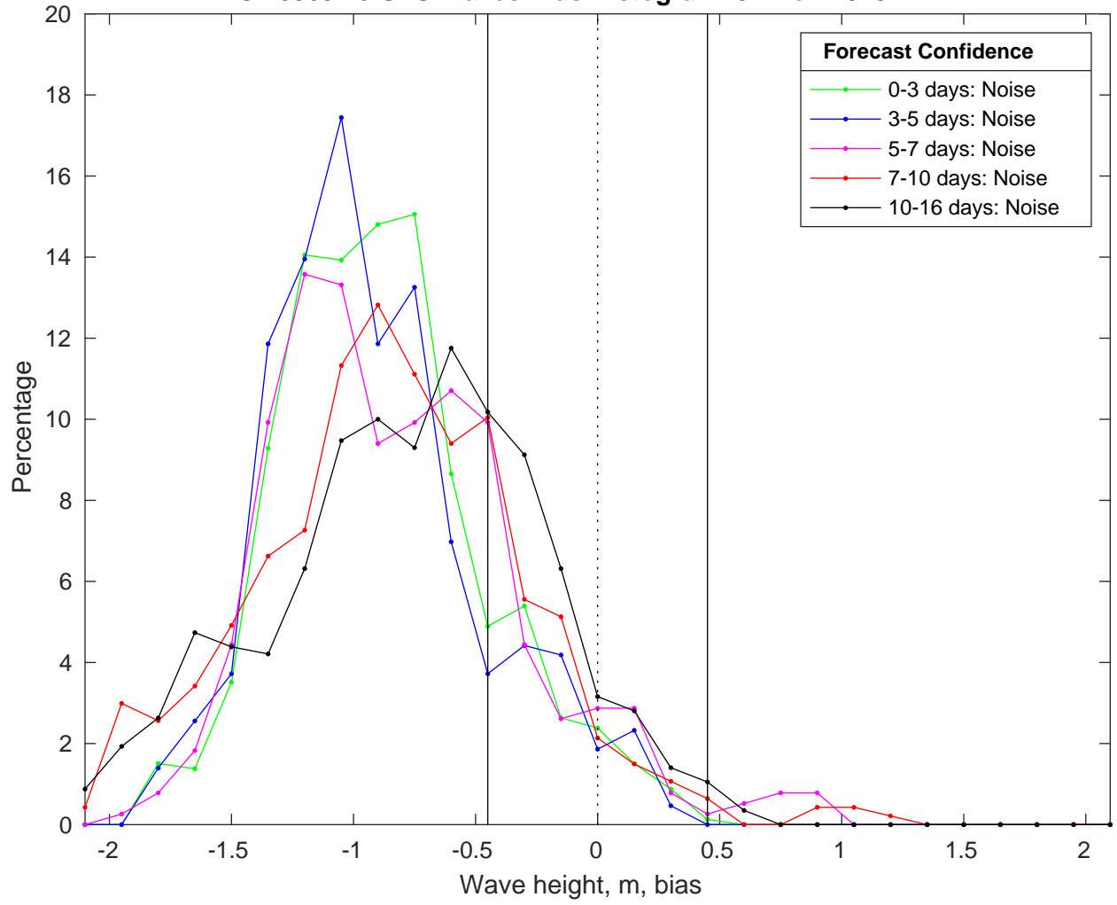
NDBC 46069 vs GFS Waves Bias Histogram: 04-Nov-2025
