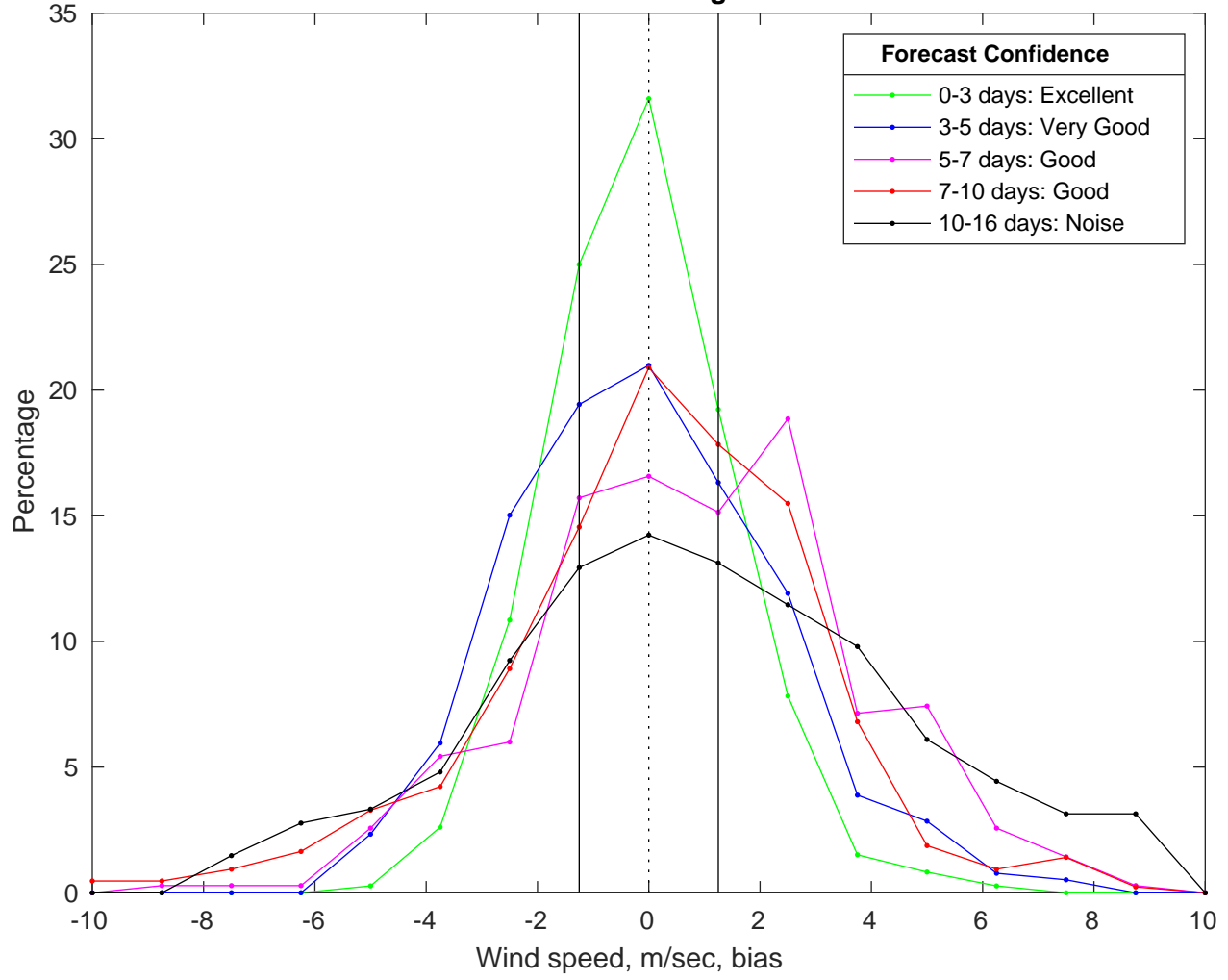
NDBC 46069 vs GFS Winds Bias Histogram: 04-Nov-2025
