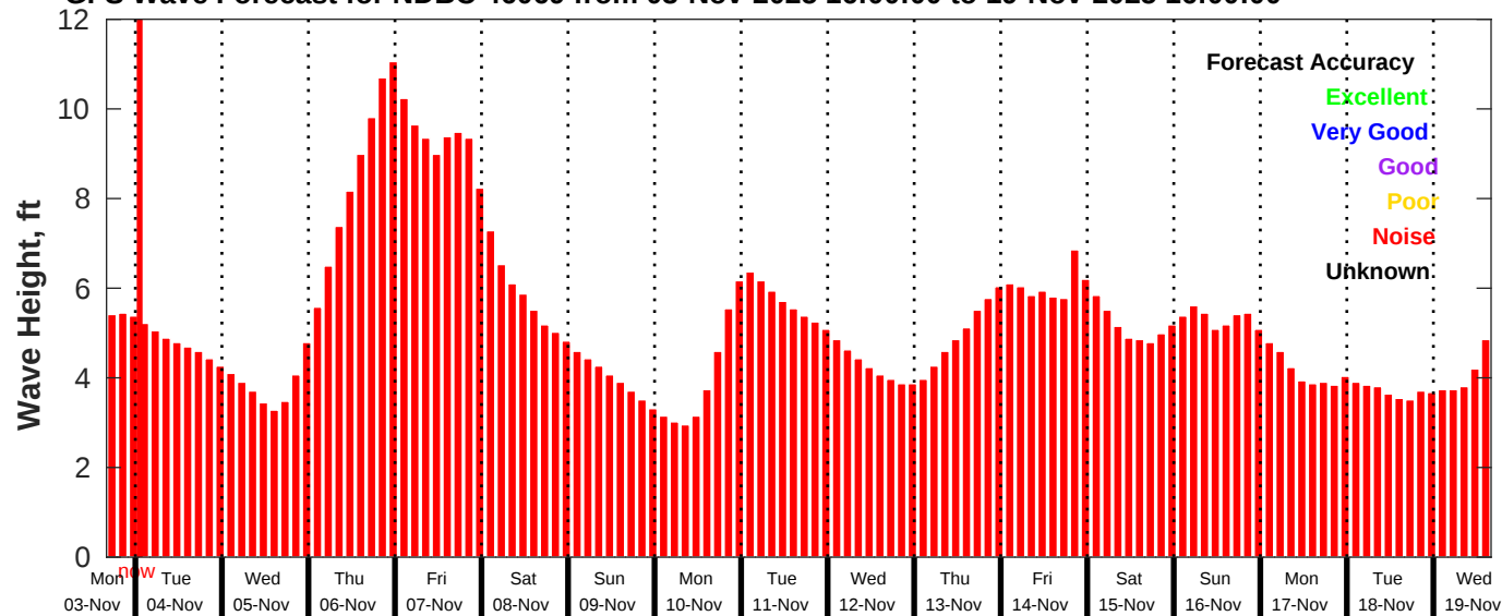
GFS Wave Forecast for NDBC 46069 from 03-Nov-2025 16:00:00 to 19-Nov-2025 16:00:00
