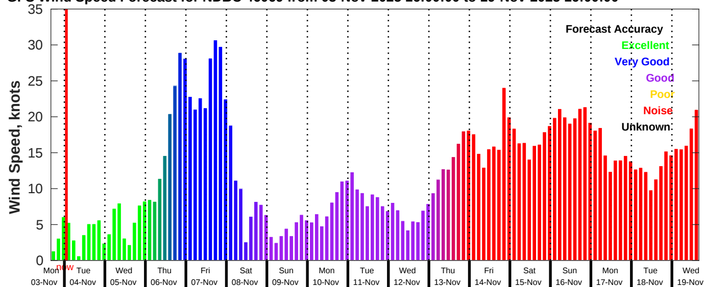
GFS Wind Speed Forecast for NDBC 46069 from 03-Nov-2025 16:00:00 to 19-Nov-2025 16:00:00
