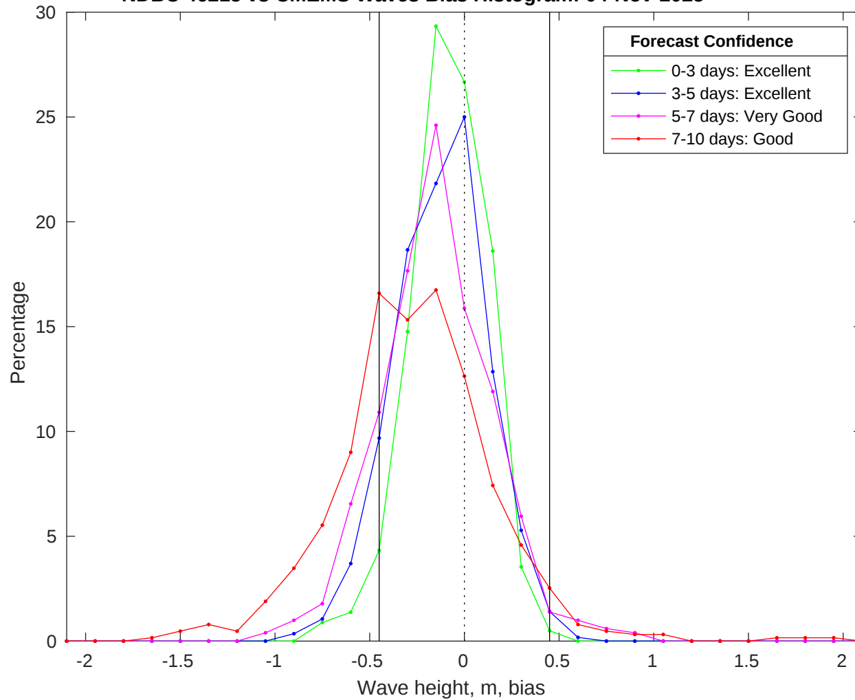
NDBC 46215 vs CMEMS Waves Bias Histogram: 04-Nov-2025
