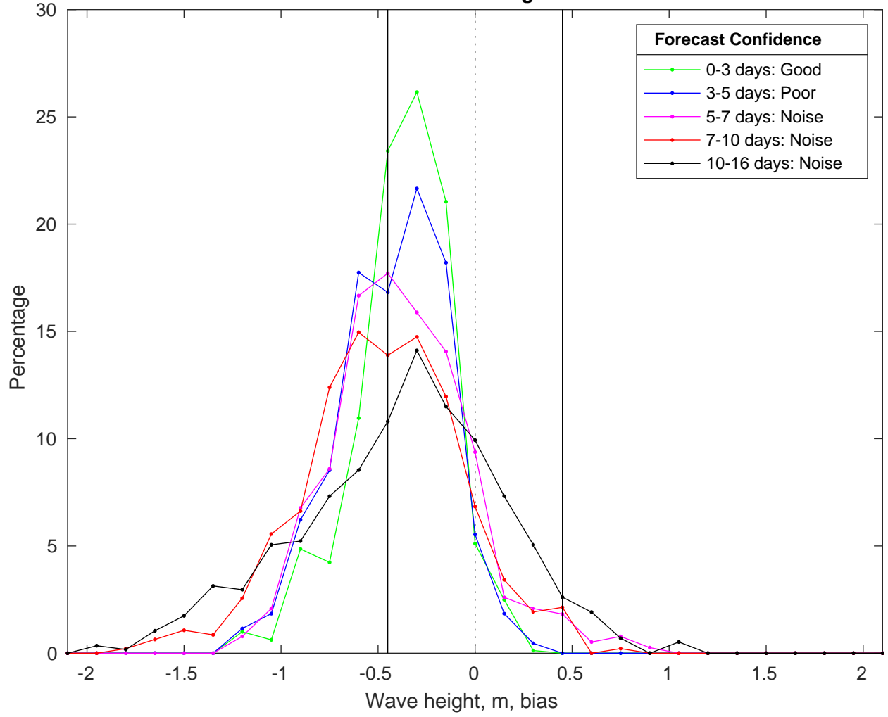
NDBC 46215 vs GFS Waves Bias Histogram: 04-Nov-2025
