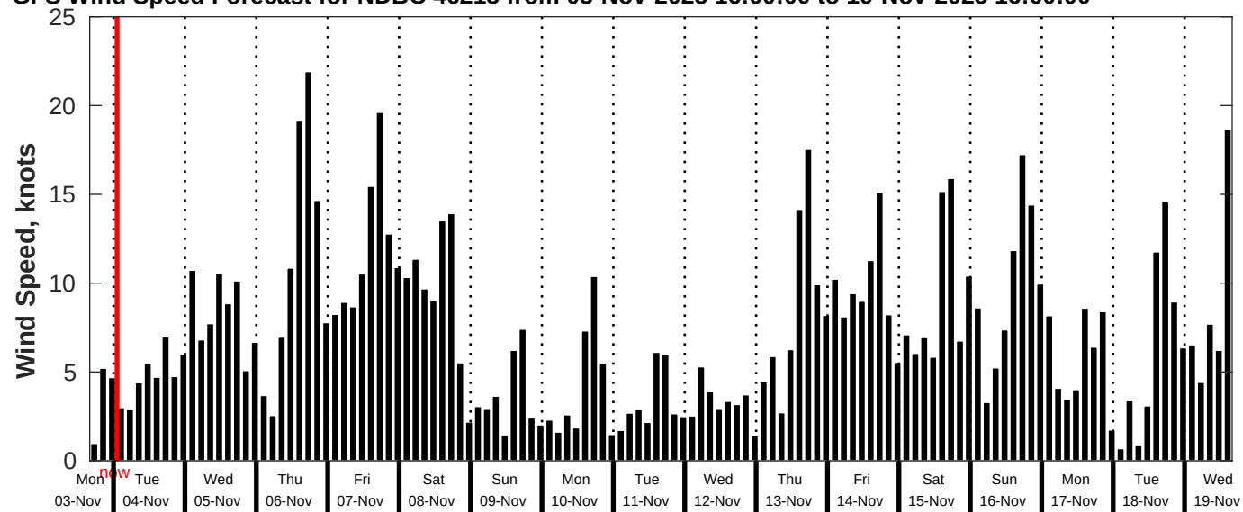
GFS Wind Speed Forecast for NDBC 46215 from 03-Nov-2025 16:00:00 to 19-Nov-2025 16:00:00
