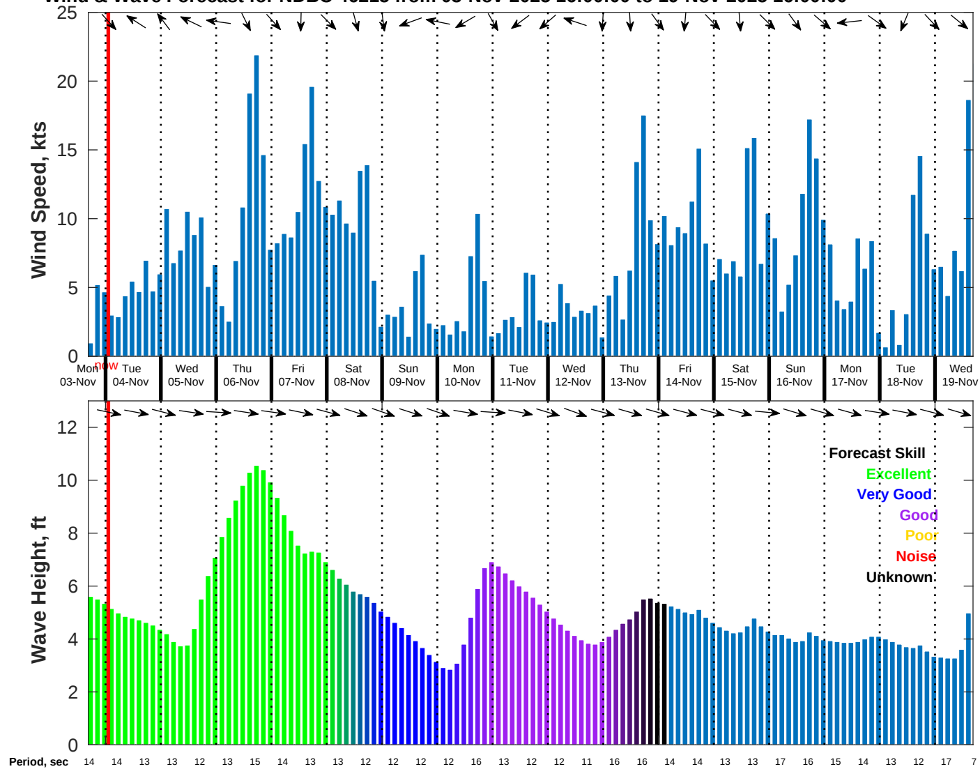
Wind & Wave Forecast for NDBC 46215 from 03-Nov-2025 16:00:00 to 19-Nov-2025 16:00:00
