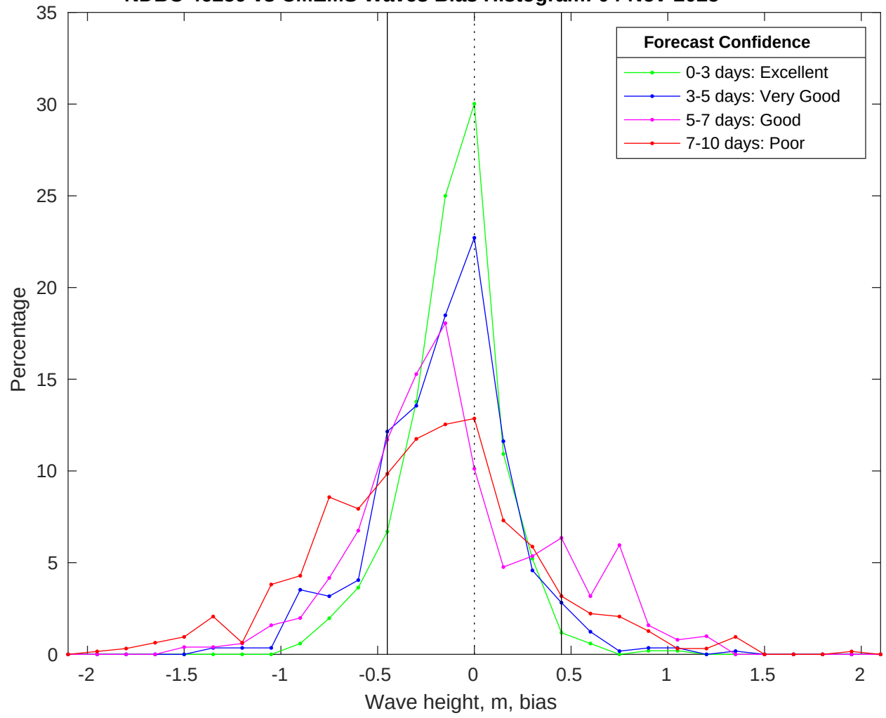
NDBC 46259 vs CMEMS Waves Bias Histogram: 04-Nov-2025
