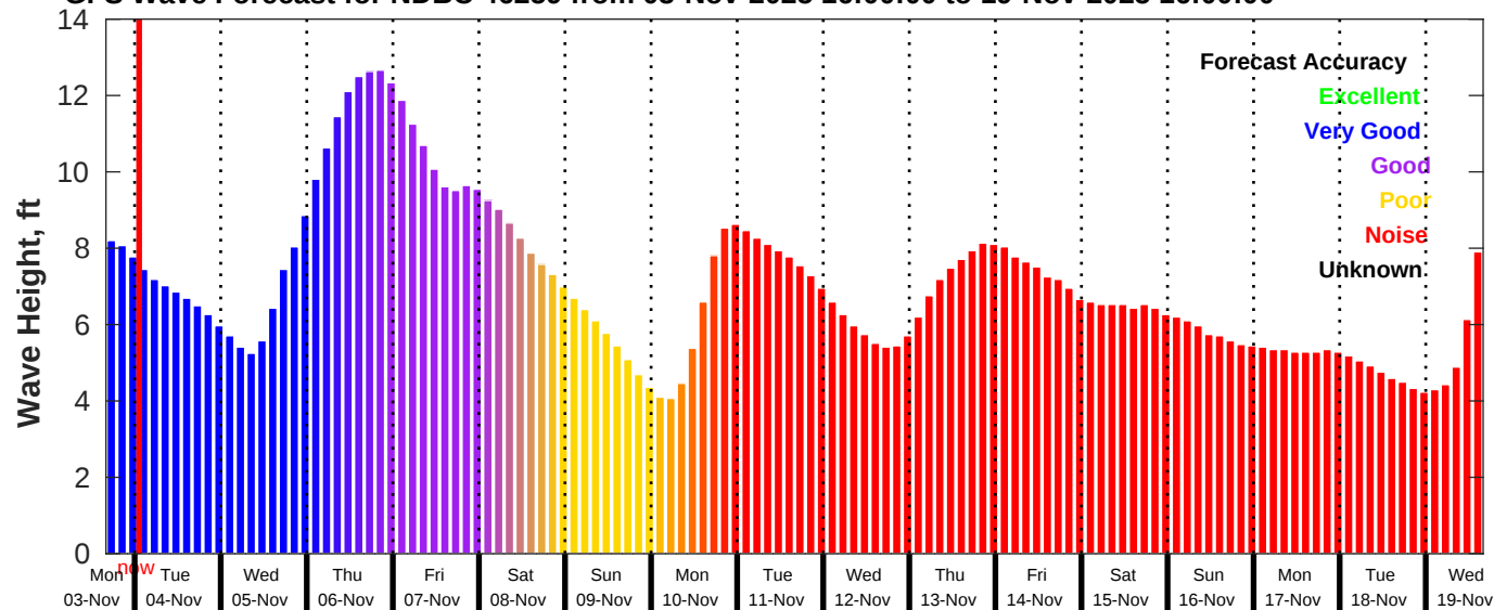
GFS Wave Forecast for NDBC 46259 from 03-Nov-2025 16:00:00 to 19-Nov-2025 16:00:00
