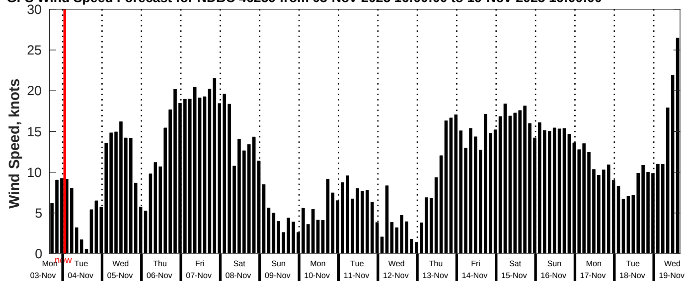
GFS Wind Speed Forecast for NDBC 46259 from 03-Nov-2025 16:00:00 to 19-Nov-2025 16:00:00
