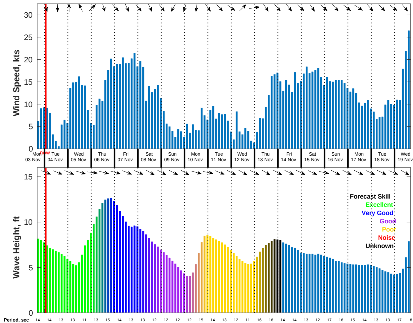
Wind & Wave Forecast for NDBC 46259 from 03-Nov-2025 16:00:00 to 19-Nov-2025 16:00:00
