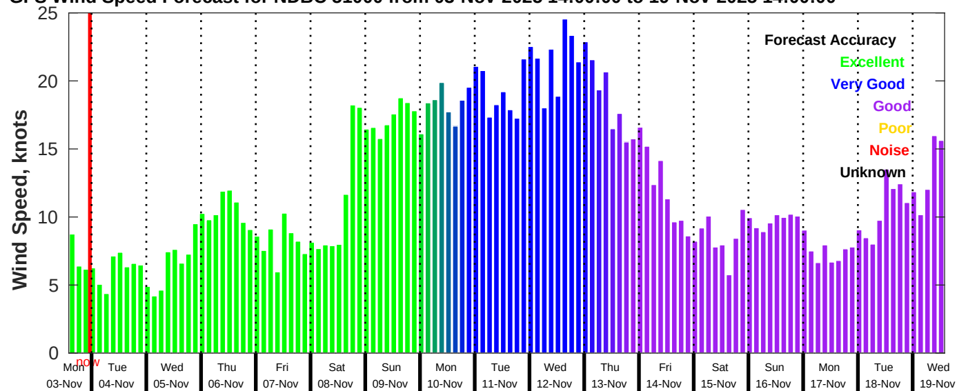
GFS Wind Speed Forecast for NDBC 51000 from 03-Nov-2025 14:00:00 to 19-Nov-2025 14:00:00
