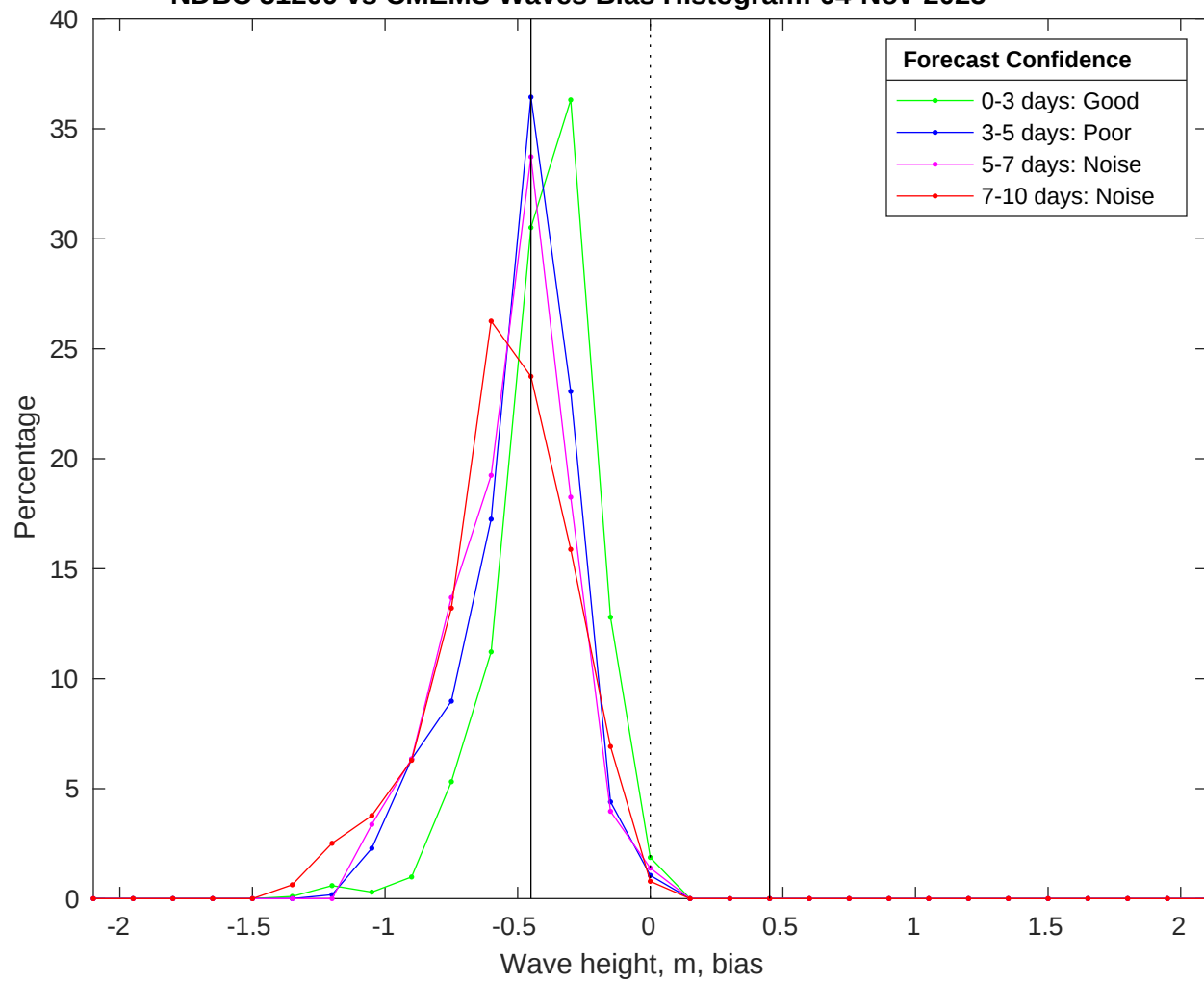
NDBC 51209 vs CMEMS Waves Bias Histogram: 04-Nov-2025
