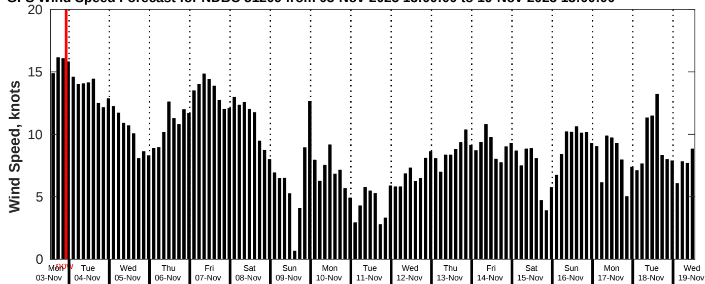
GFS Wind Speed Forecast for NDBC 51209 from 03-Nov-2025 13:00:00 to 19-Nov-2025 13:00:00
