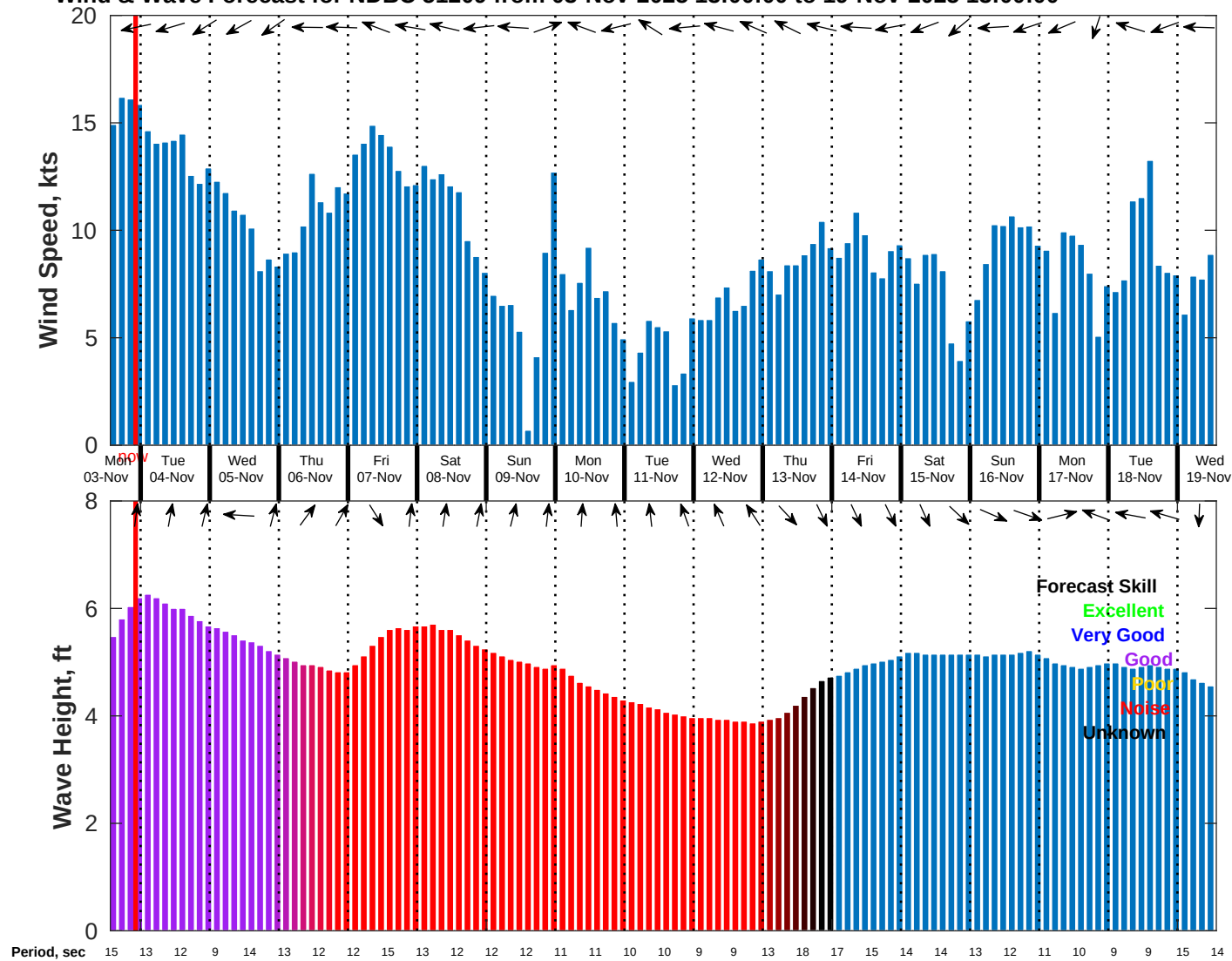
Wind & Wave Forecast for NDBC 51209 from 03-Nov-2025 13:00:00 to 19-Nov-2025 13:00:00
