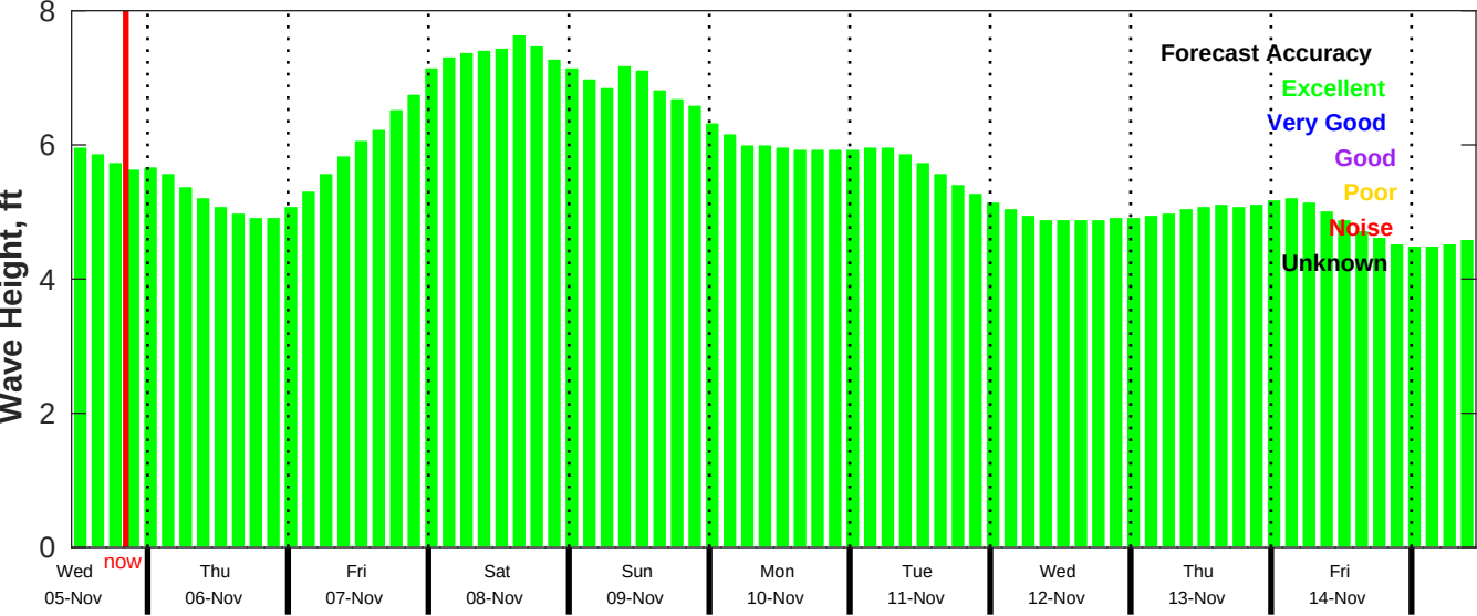
CMEMS Wave Forecast for NDBC 52211 from 04-Nov-2025 11:00:00 to 14-Nov-2025 11:00:00
