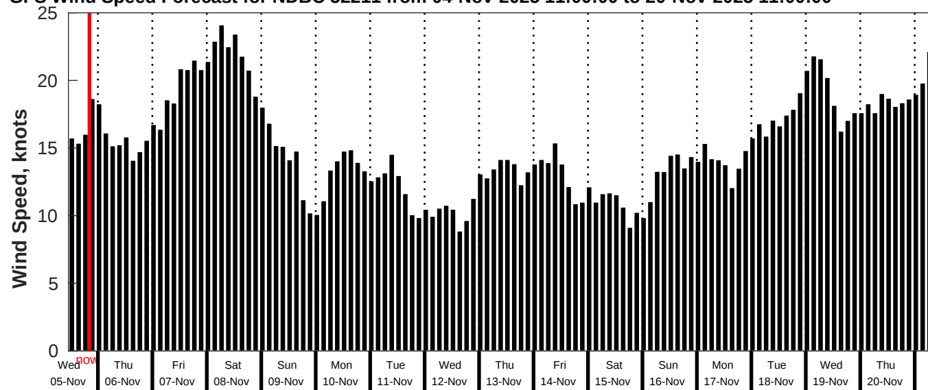
GFS Wind Speed Forecast for NDBC 52211 from 04-Nov-2025 11:00:00 to 20-Nov-2025 11:00:00
