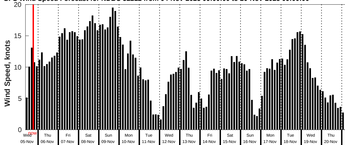
GFS Wind Speed Forecast for NDBC 52212 from 04-Nov-2025 09:00:00 to 20-Nov-2025 09:00:00
