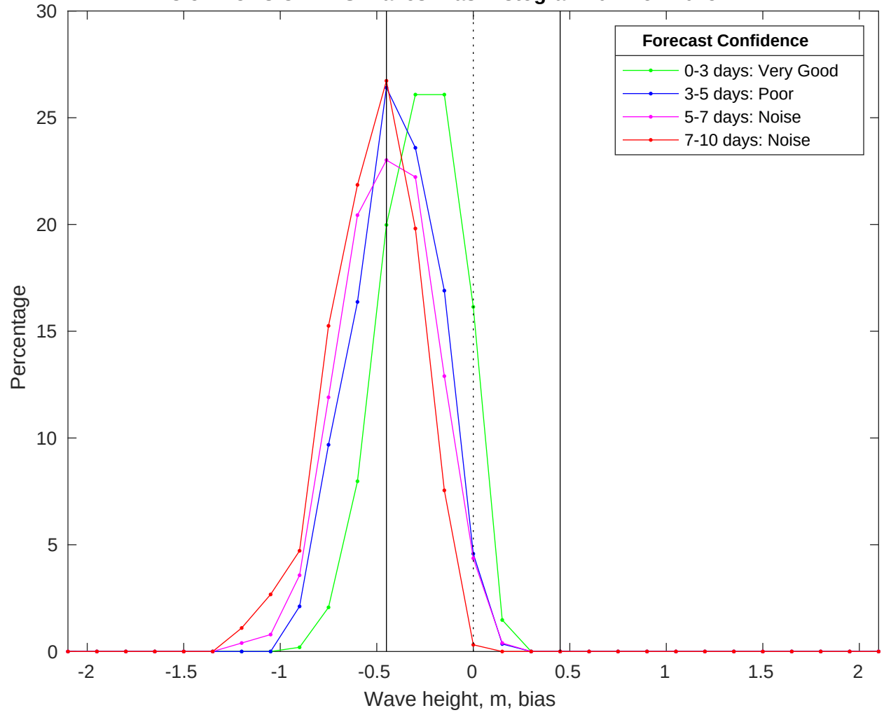
NDBC 52213 vs CMEMS Waves Bias Histogram: 04-Nov-2025
