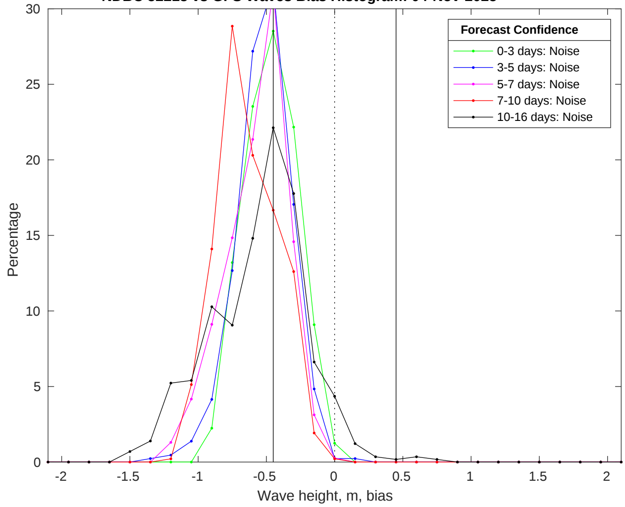
NDBC 52213 vs GFS Waves Bias Histogram: 04-Nov-2025
