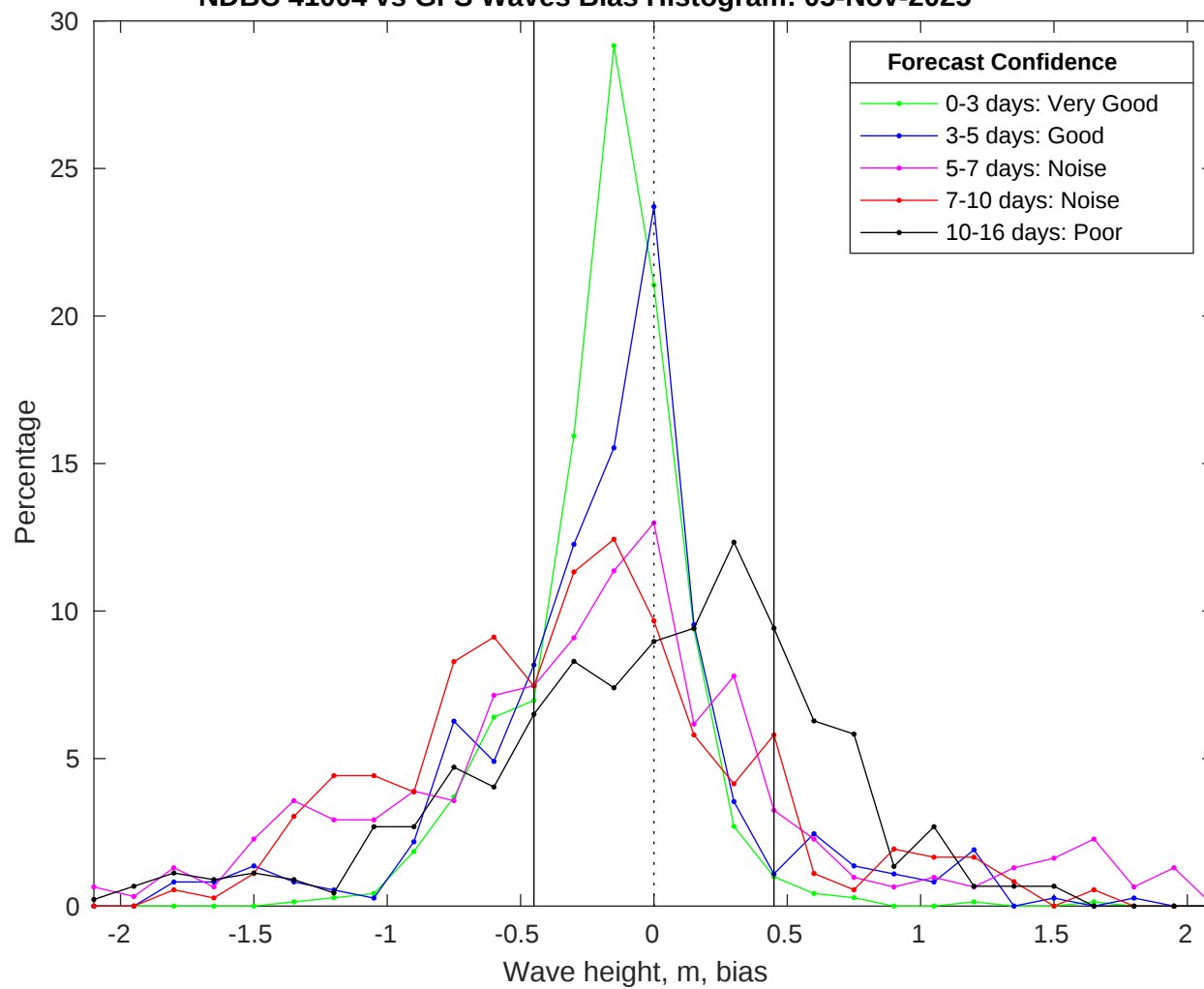
NDBC 41004 vs GFS Waves Bias Histogram: 05-Nov-2025
