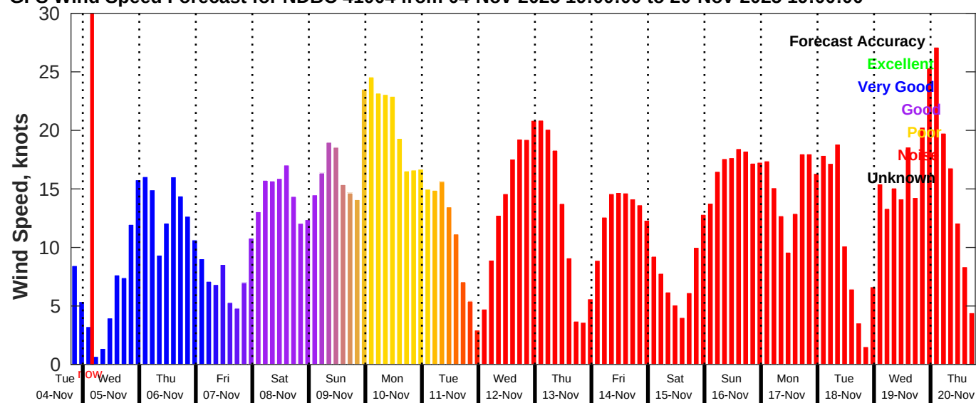
GFS Wind Speed Forecast for NDBC 41004 from 04-Nov-2025 19:00:00 to 20-Nov-2025 19:00:00
