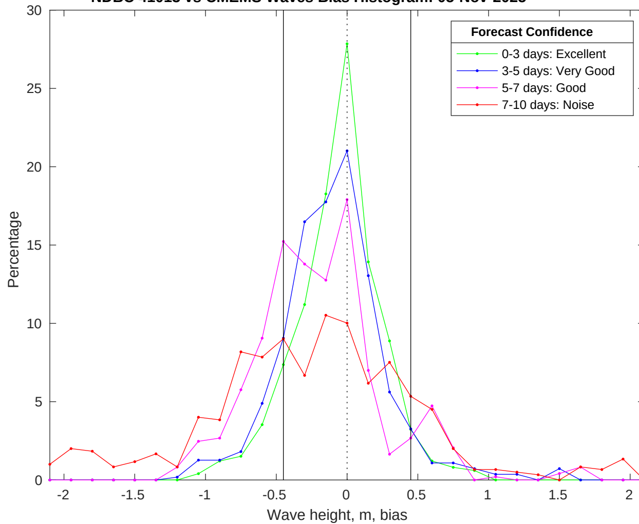
NDBC 41013 vs CMEMS Waves Bias Histogram: 05-Nov-2025
