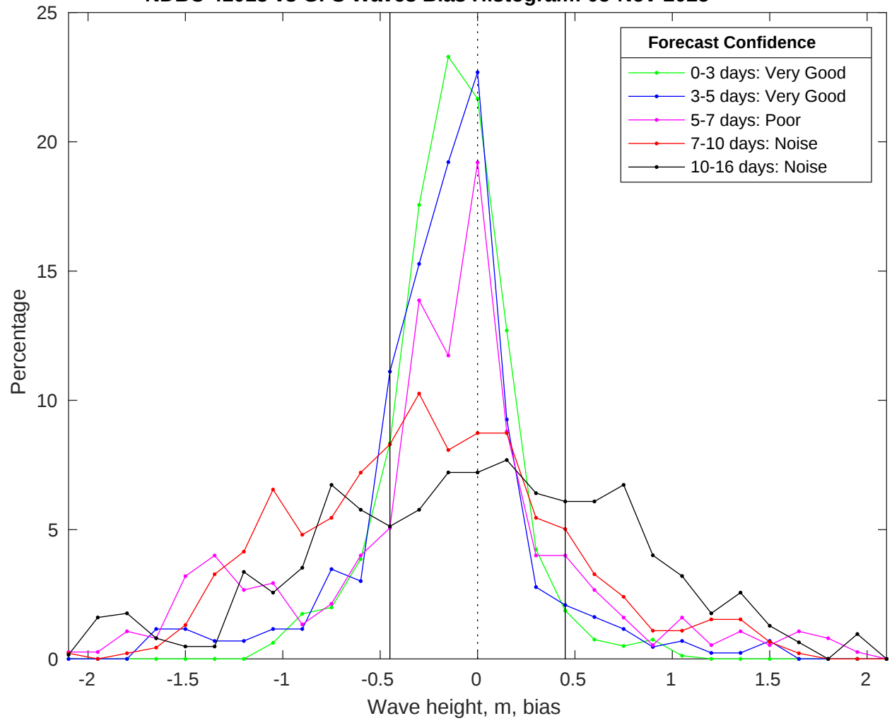
NDBC 41013 vs GFS Waves Bias Histogram: 05-Nov-2025
