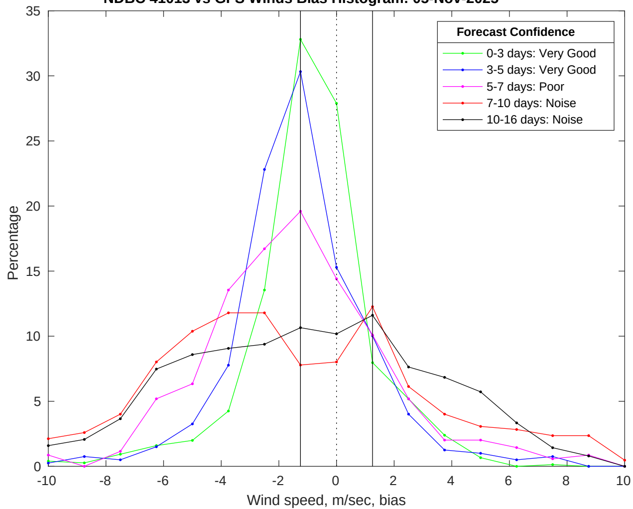
NDBC 41013 vs GFS Winds Bias Histogram: 05-Nov-2025
