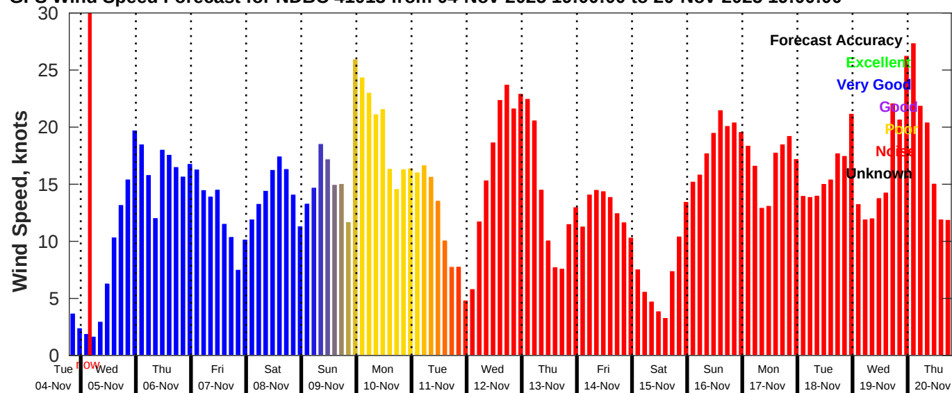
GFS Wind Speed Forecast for NDBC 41013 from 04-Nov-2025 19:00:00 to 20-Nov-2025 19:00:00
